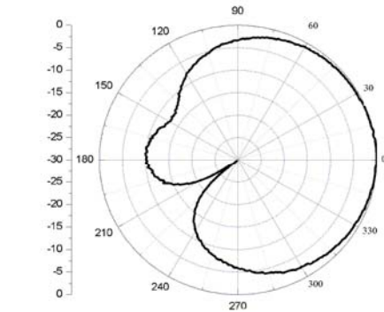
H Plane
