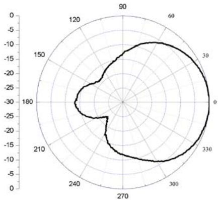
E Plane
