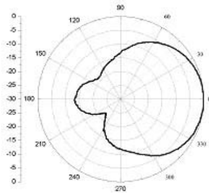
E Plane
