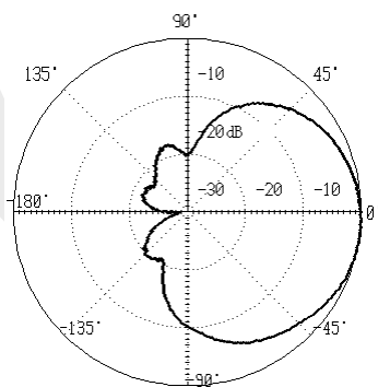
Frequency = 2GHz
