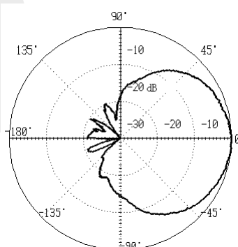
Frequency = 10GHz
