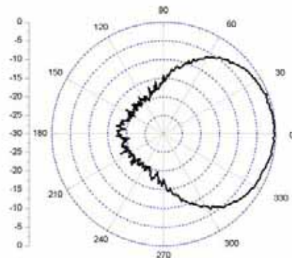
E Plane
