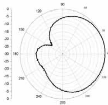
H Plane
