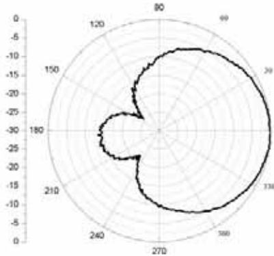
E Plane
