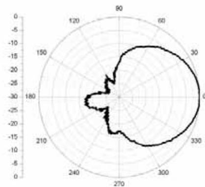
H Plane
